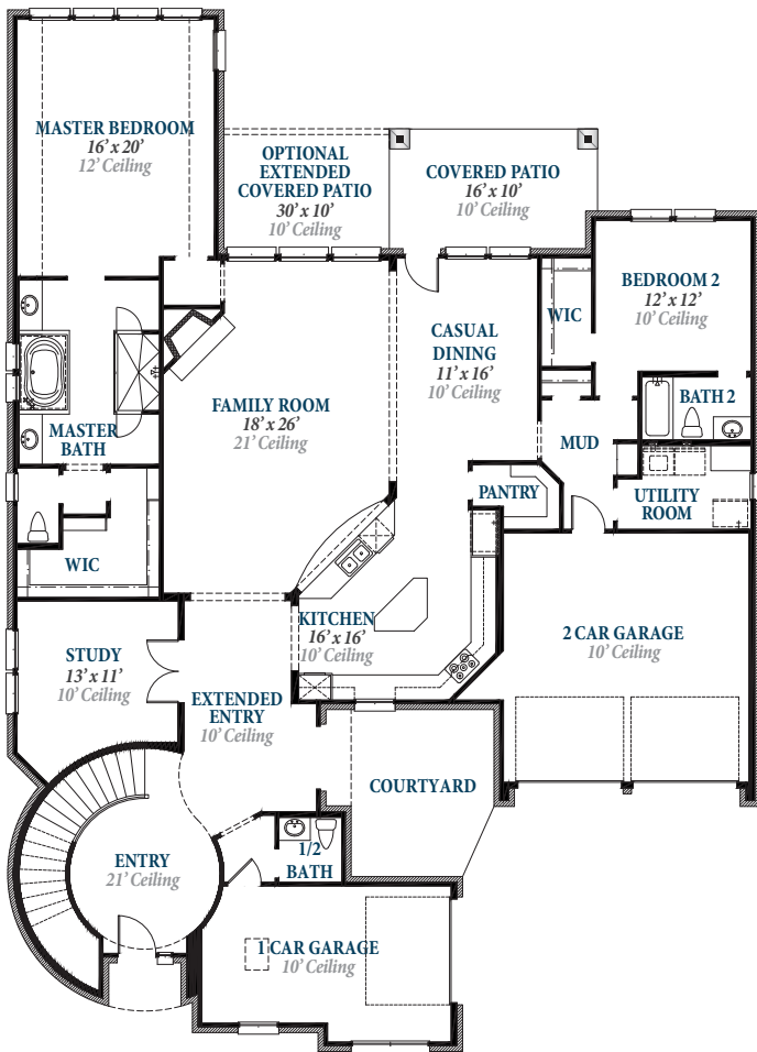
• FIRST FLOOR •
