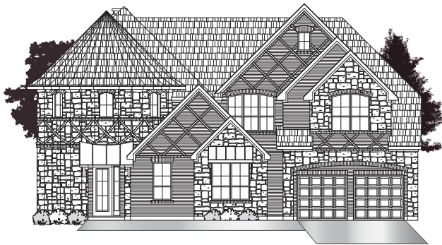
• ELEVATION B1 •
